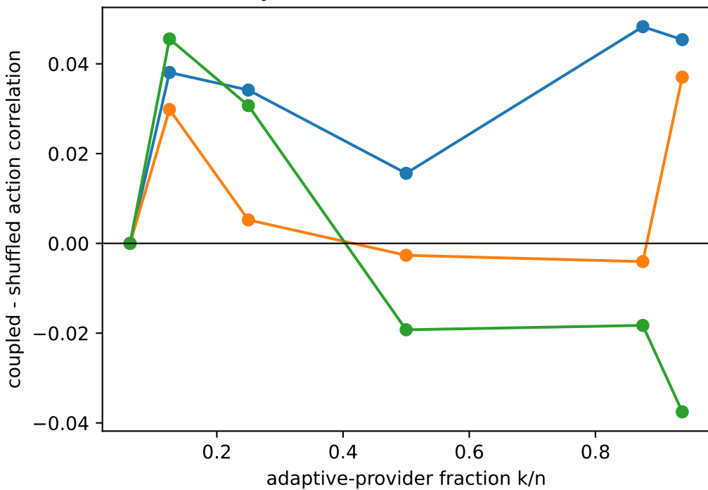
C. Synthetic coordination channel
