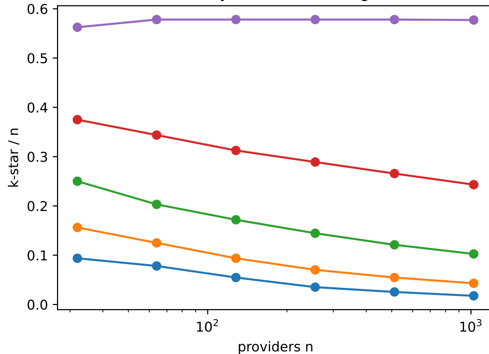
D. Synthetic allocation effect
