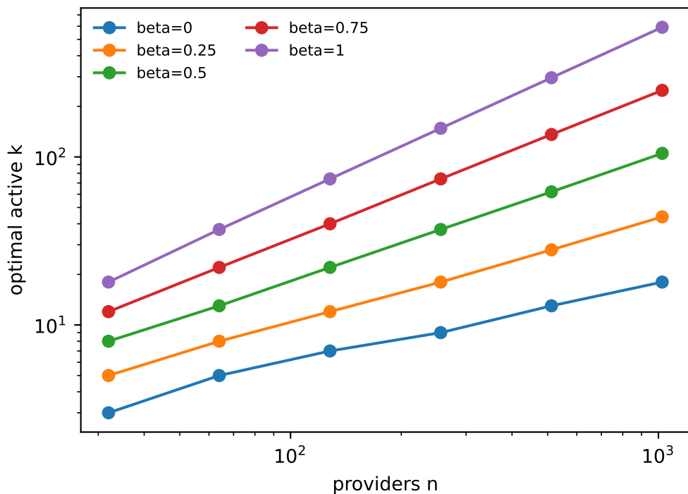
C. Synthetic coordination channel
