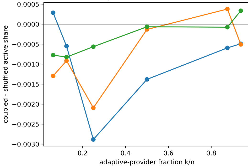
D. Synthetic allocation effect
