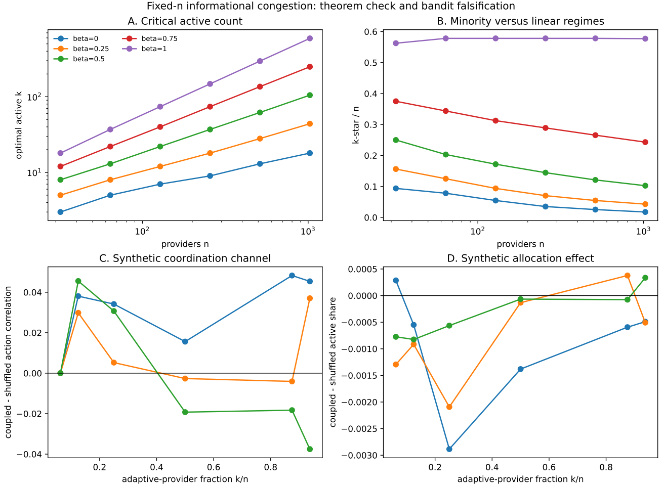
Figure 2: Fixed- n information-congestion check and behavioral falsification. Panels A–B recover the conditional optimizer in theorem 6. Panels C–D show that the marginal-preserving signal intervention can alter simulated action correlation while its active-share effect remains economically and statistically indistinguishable from zero. Theory recovery is not evidence that the declared bandit generates the loss.
