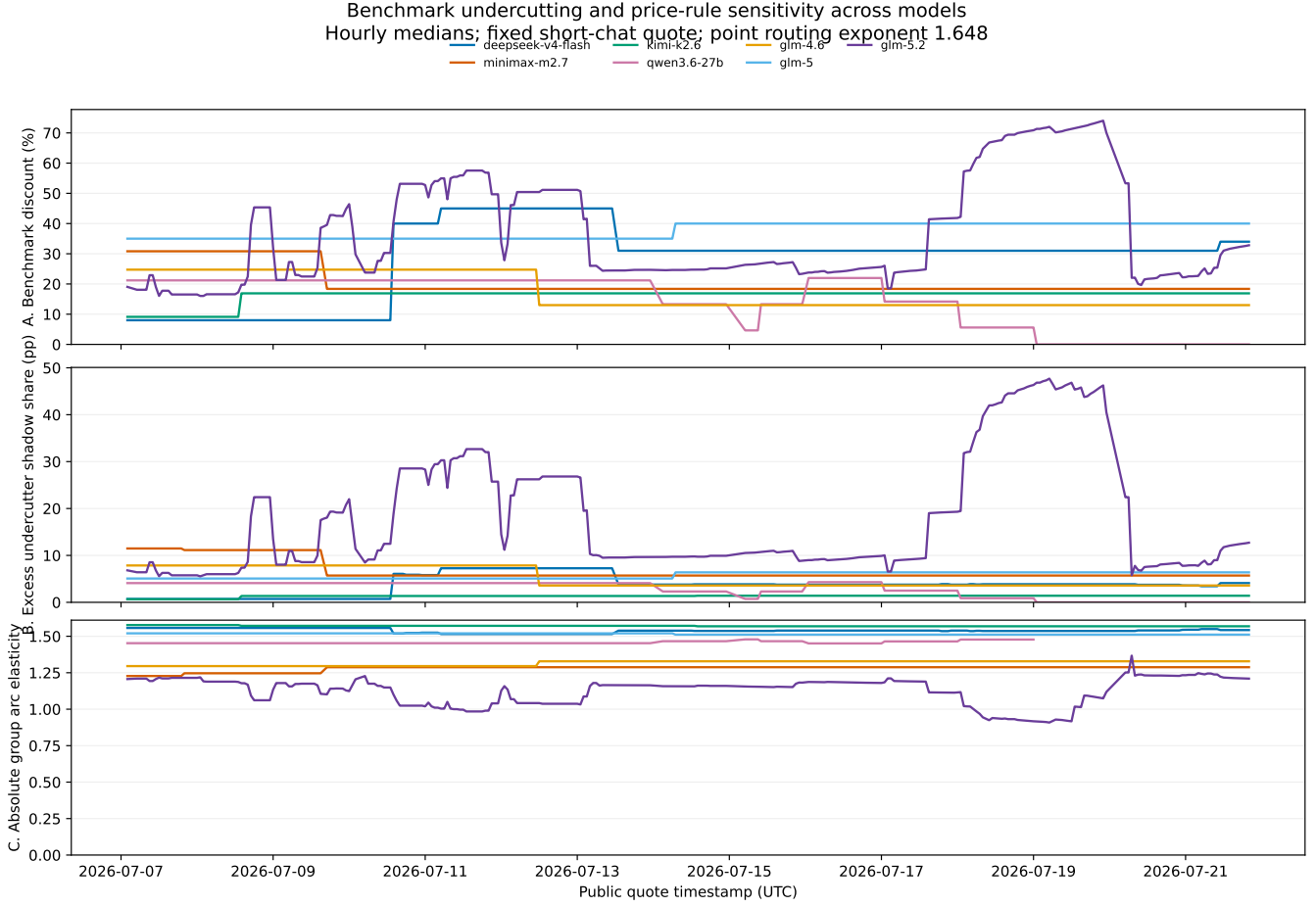
Figure 2: Time variation in the displayed-price mechanism. Hourly medians put all seven models on the same axes. GLM-5.2 is both the most variable series and the largest mechanical transfer surface, while most other menus move in discrete regimes. Panel C is the price-rule arc elasticity at the frozen point exponent; it is not a realized-demand estimate. Free endpoints are excluded because a zero quote makes the inverse-power counterfactual undefined.
