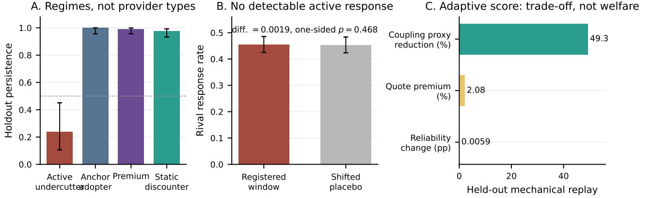
Figure 3: Three empirical boundaries. Panel A: frozen training regimes and holdout persistence (Wilson 95% intervals). Panel B: active-undercutter rival response in the registered window versus a shifted timing placebo. Panel C: held-out adaptive-score replay; the reliability change is in percentage points. Panel C holds menus and provider behavior fixed, so it is not a welfare estimate.
