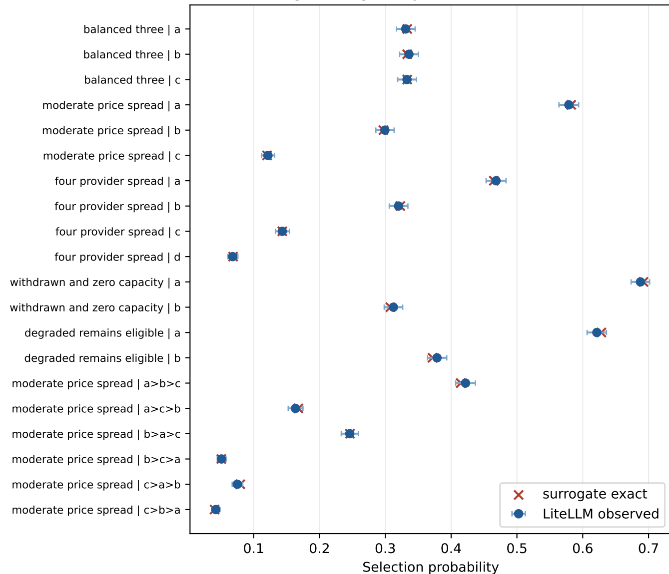
Exact target and globally simultaneous 95% interval
