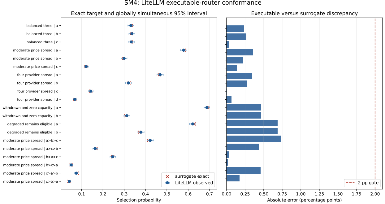
Figure 1: Executable LiteLLM conformance. Crosses are exact surrogate probabilities; dots and bars are LiteLLM frequencies and globally simultaneous 95% intervals. The bottom six rows are complete fallback permutations, not independent first-route draws.
