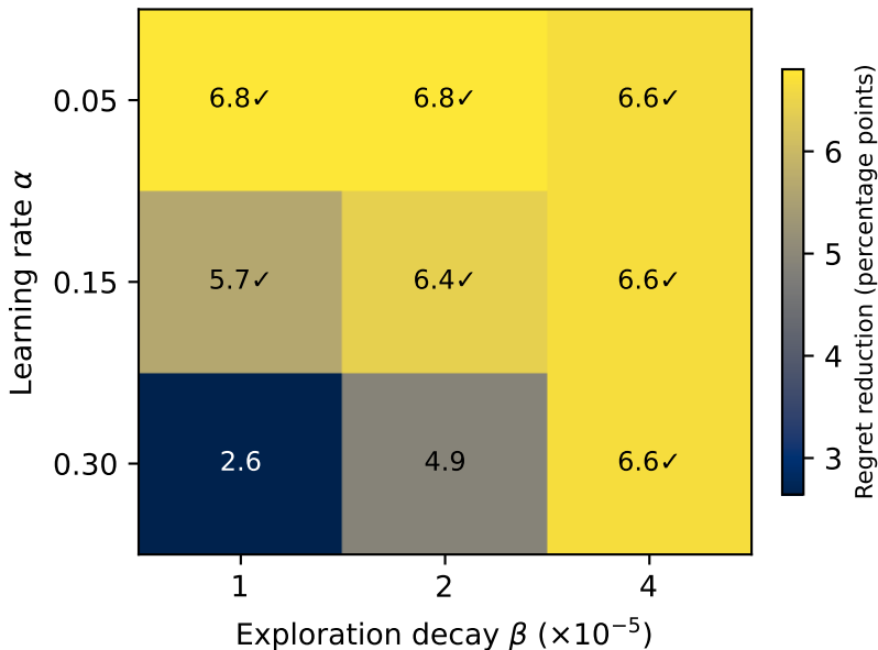
Option lowers regret in all cells
