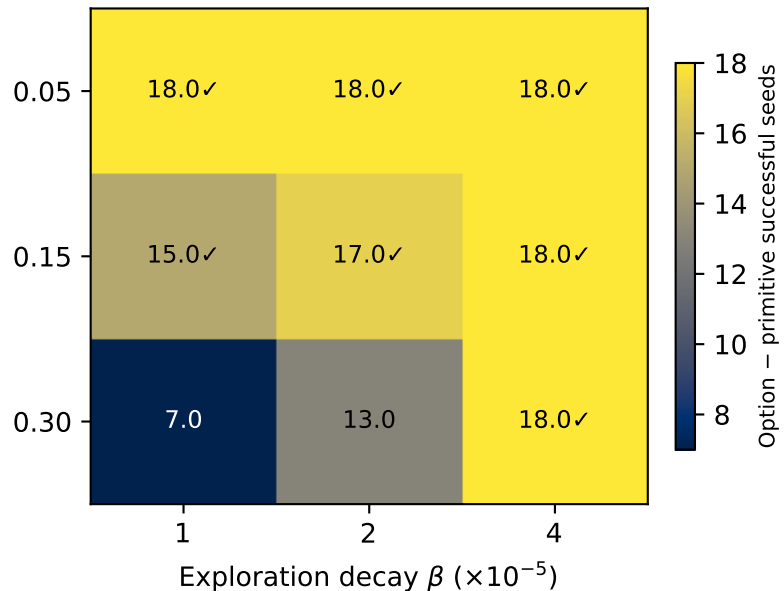
Primitive failure depends on learning rate
