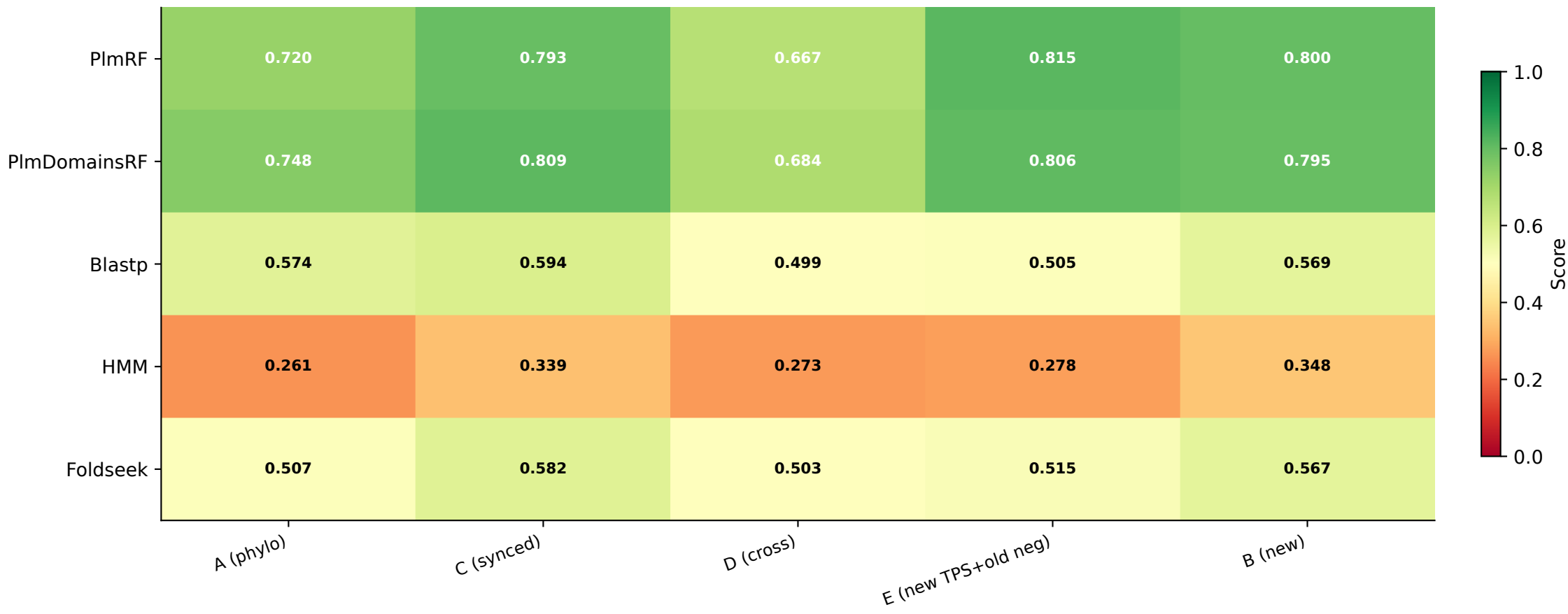
Substrate Prediction — Major Substrates (mAP)
