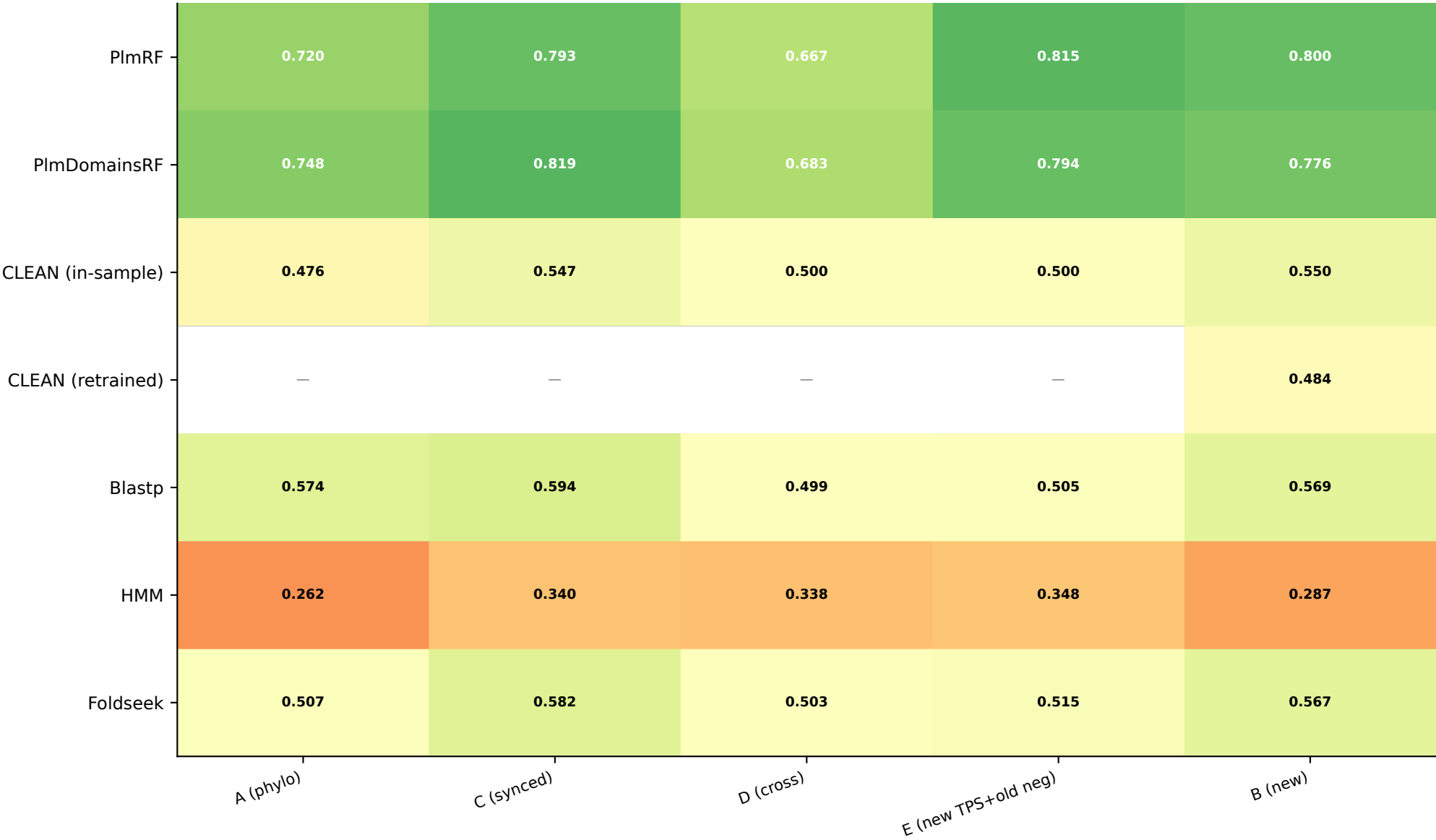
Substrate Prediction — Major Substrates (mAP)
