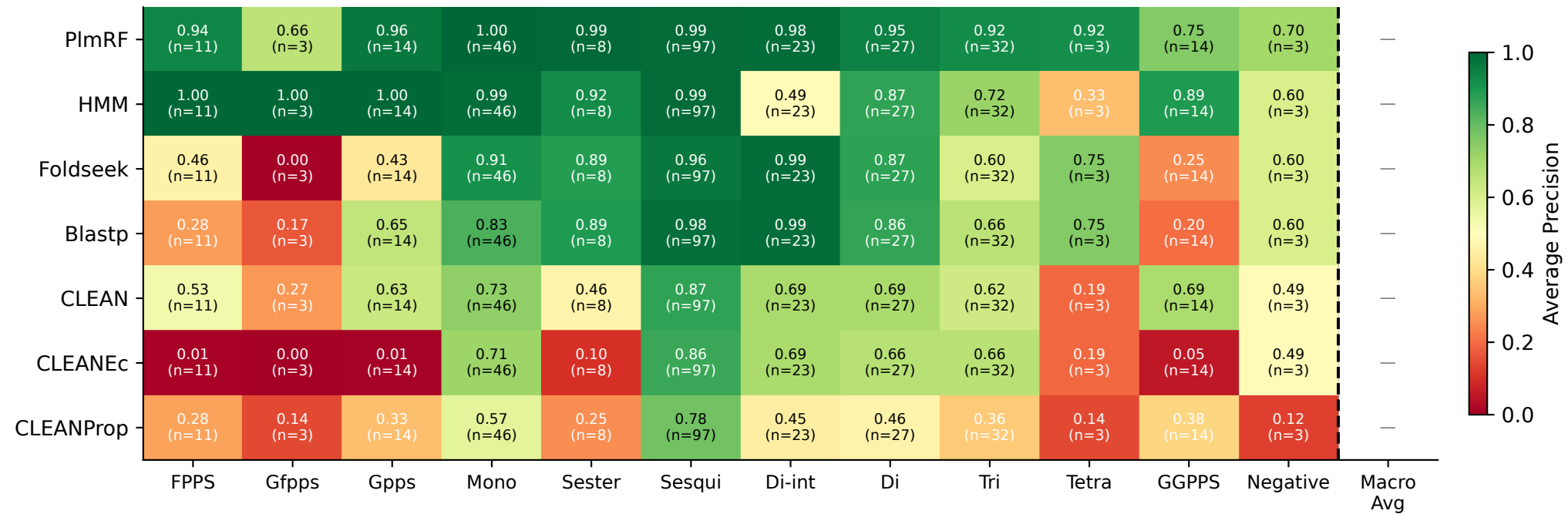
Per-Type TPS Detection AP — Track A
