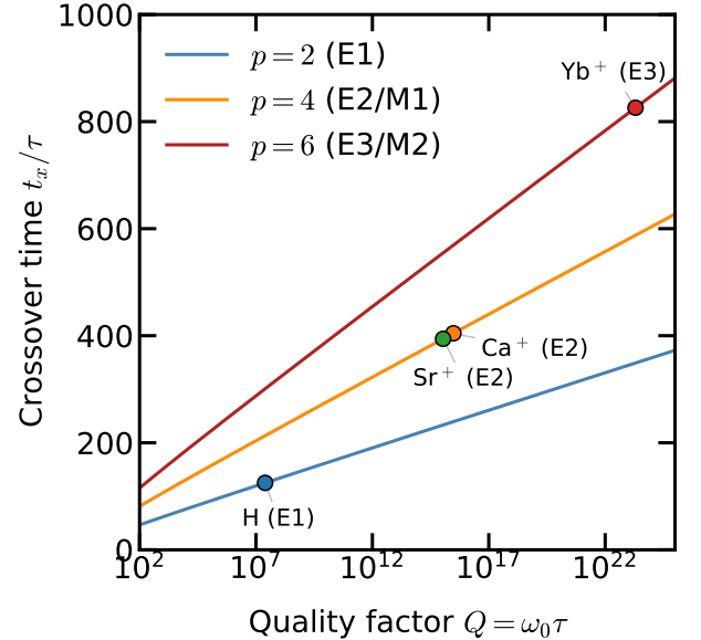
FIG. 1. Envelope exponential-to-power-law turnover time t_x/\tau as a function of the quality factor Q = \omega_0 \tau , where \omega_0 is the atomic transition frequency and \tau = 1/\Gamma is the lifetime. The solid curves show the asymptotic estimate used in these notes, where p is the multipole exponent of the late-time tail. Markers indicate the real transitions of Table I. EL (ML) indicates the electric (magnetic) character of the transition with multipole order L .
