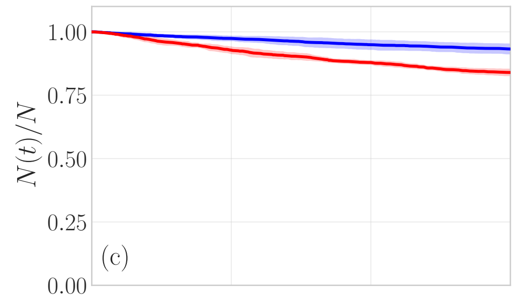
Effective network size: N(t)/N
