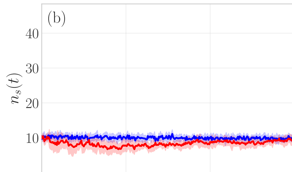
Number of communities: n_s(t)
