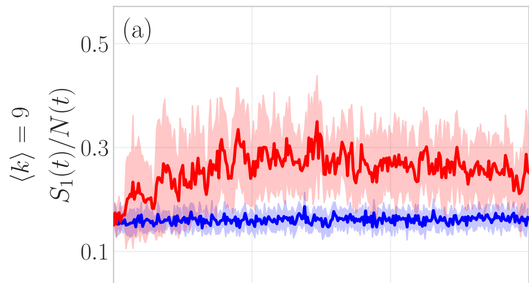
Largest community: S_1(t)/N(t)
