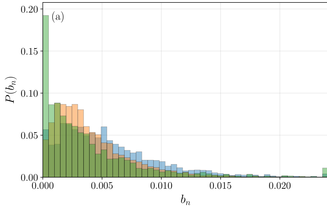
Node betweenness
