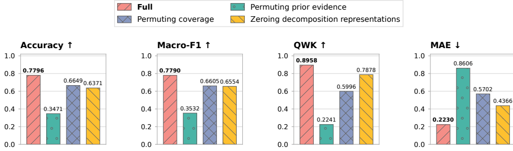
Figure 2: Pipeline-stage ablations on IdeaDelta. Full is the unablated checkpoint of Table 1; each intervention is applied at inference without retraining. Arrows indicate the preferred direction for each metric.
