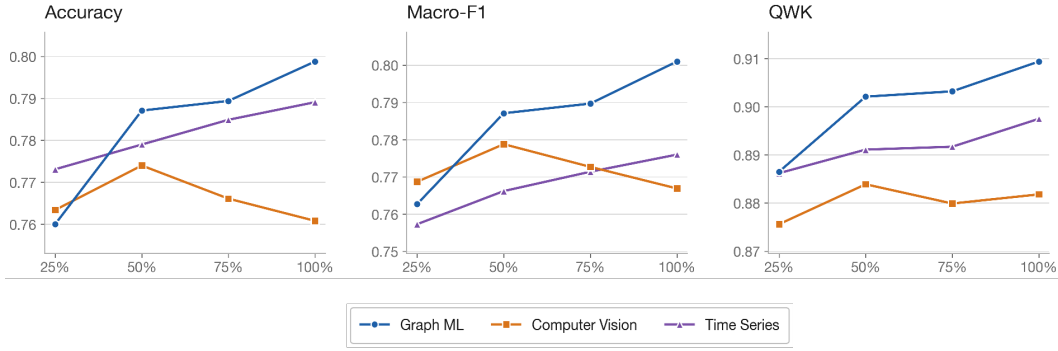
Figure 6: Sensitivity to the amount of EGRD training data in the three domains. Development and test sets stay fixed, and 100% is the default.
