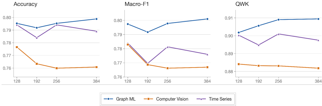
Figure 7: Sensitivity to encoder input length on the three domain test splits. The default is 384, and every setting scores the same test ideas and labels.
