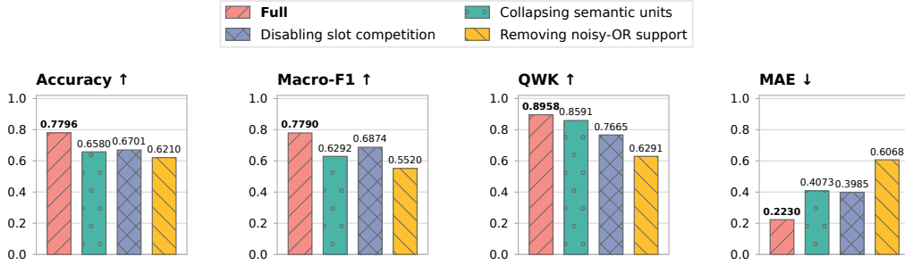
Figure 2: Pipeline-stage ablations on IdeaDelta. Full is the unablated checkpoint of Table 1; each intervention is applied at inference without retraining. Arrows indicate the preferred direction for each metric.
