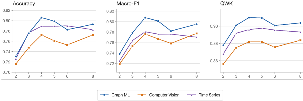
Figure 5: Sensitivity to the evidence budget K in the three domains. The default is K=5 , the checkpoint of Table 1. K specifies the number of input slots, including padding when fewer priors are available.
