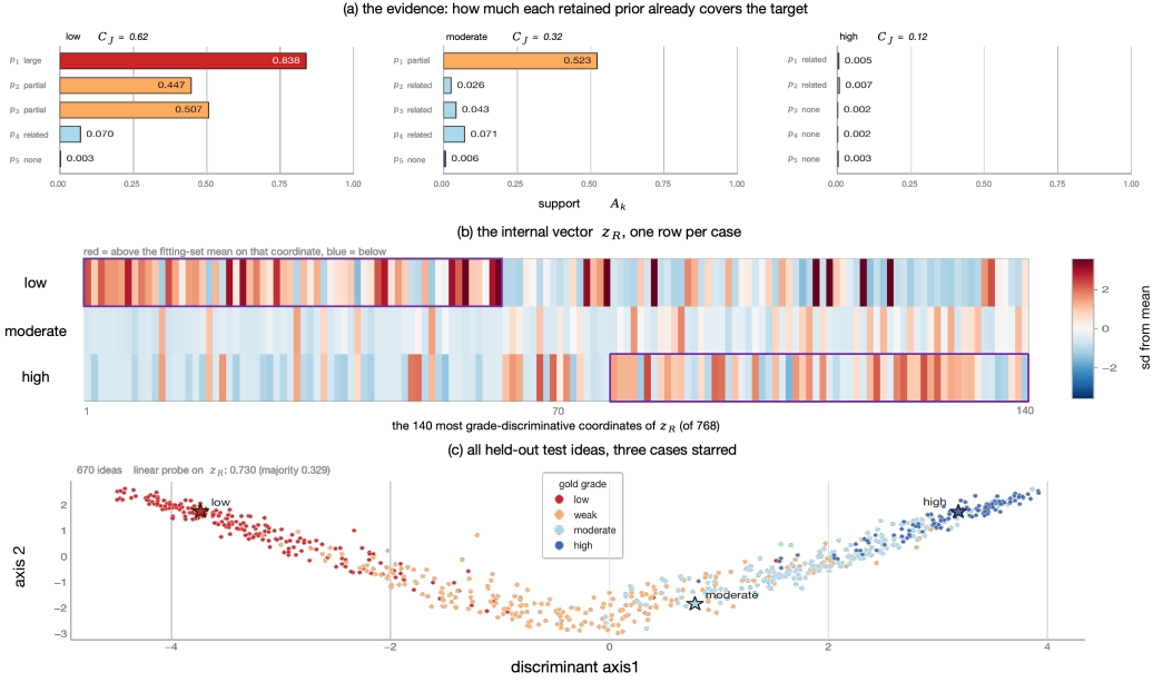
Figure 4: Three test targets, graded low, moderate and high, traced through the model. (a) The support A_k assigned to each retained prior, against the coverage label the annotation carries; C_J is the predicted joint coverage. (b) The residual representation z_R of each case, as deviations from the fitting-set mean. (c) z_R for every held-out test idea, coloured by gold grade, the three cases starred.
