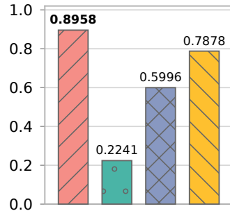
QWK ↑
