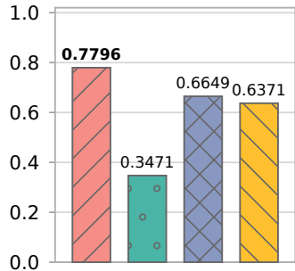
Accuracy ↑
