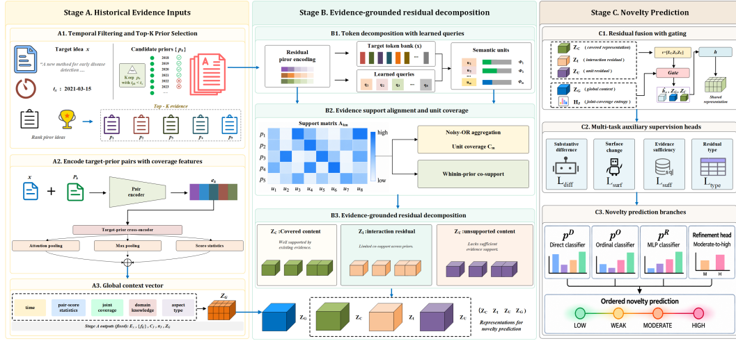
Figure 2: Overview of EGRD. (A) Only priors predating the target are admissible; the retained top- K evidence carries pair coverage features f_k , and a multiple-instance model predicts joint coverage C_J and its four-class distribution \pi^J . Stage A outputs enter the later stages as fixed inputs, marked sg[\cdot] . (B) M learned queries partition a target token bank into semantic units u_m ; a support matrix A_{km} aligns each unit with each prior, yielding the unit residual z_U , the covered pooling z_C , and the interaction residual z_I , which uses co-support \bar{A}_{ij} . (C) A gate modulates global context within residual fusion; the shared representation feeds three novelty branches and the moderate-to-high refinement, while the continuous score head supplies training supervision only.
