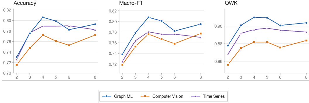
Figure 3: Sensitivity to the evidence budget K in the three domains. The default is K=5 , the checkpoint of Table 1. K is a padding dimension, so the text reads the curves against the priors each setting consumes.
