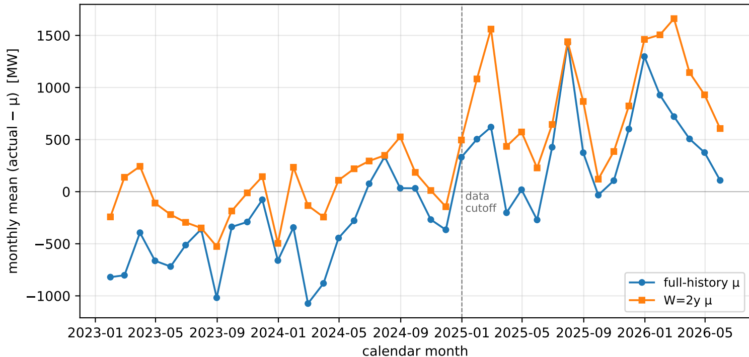
Post-cutoff climatology gap is non-stationary (no recency window can fix this)
