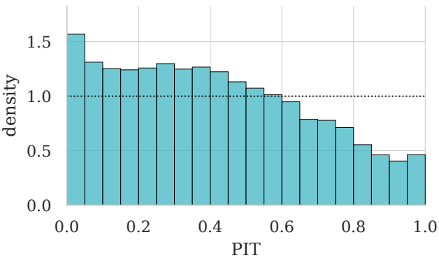
predictor 5
