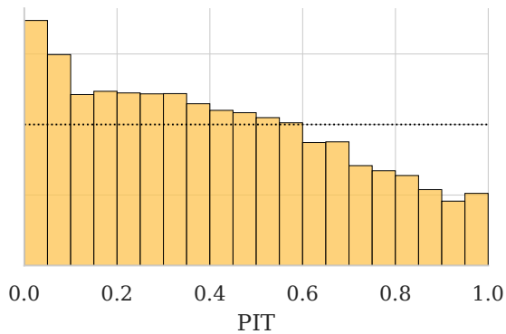
predictor 6
