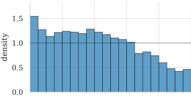
predictor 5
