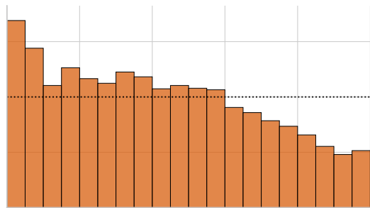
predictor 4
