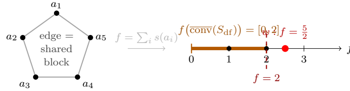
FIGURE 3. Wright’s pentagon (a Greechie 5-loop; left), and the same hull-membership question read off a separating functional (right). The state space is 5-dimensional and undrawable, but f(s) = \sum_i s(a_i) projects it faithfully to \mathbb{R} : every dispersion-free state has f \leq 2 (the odd loop admits no two adjacent atoms valued 1), so f(\overline{\text{conv}}(S_{\text{df}})) = [0, 2] . The non-classical state w \equiv \frac{1}{2} has f = \frac{5}{2} , past the face f = 2 , hence outside the hull — contextual. (Here f is a chosen separating functional for this w ; by the separating-hyperplane theorem a state is contextual iff some linear functional sends it past the hull’s image.)
