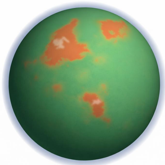
Early Archean
