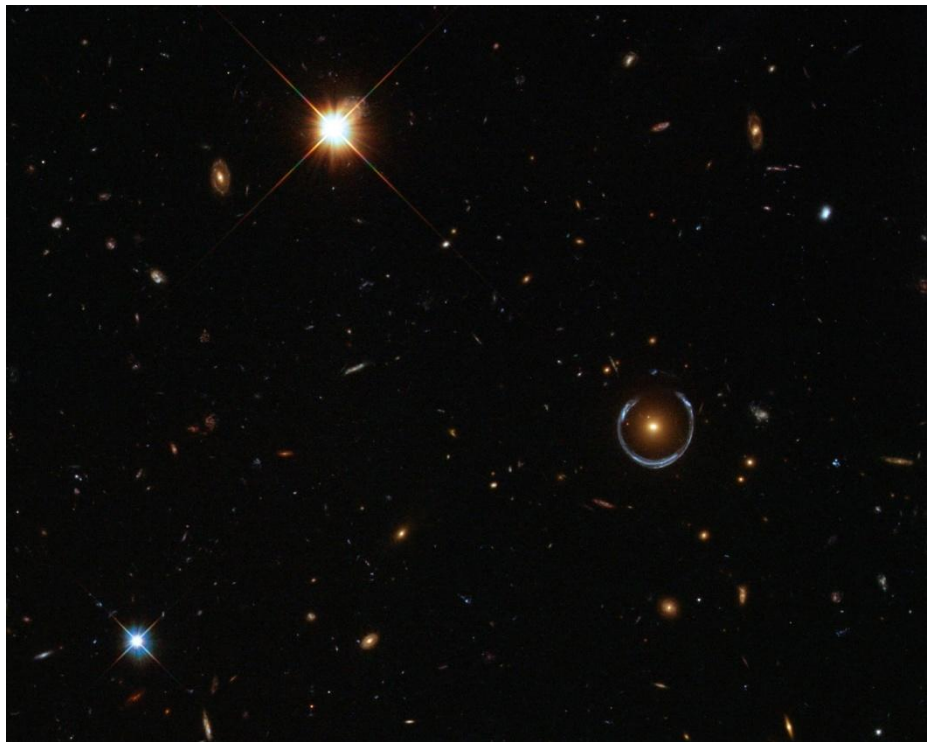
A Horseshoe Einstein Ring from Hubble Image Credit: ESA/Hubble & NASA
