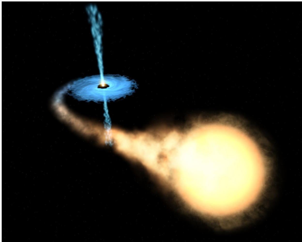
Artist's impression of the microquasar GRO J1655–40, showing a stellar-mass black hole accreting matter from a companion star, forming an accretion disk and relativistic jets.
