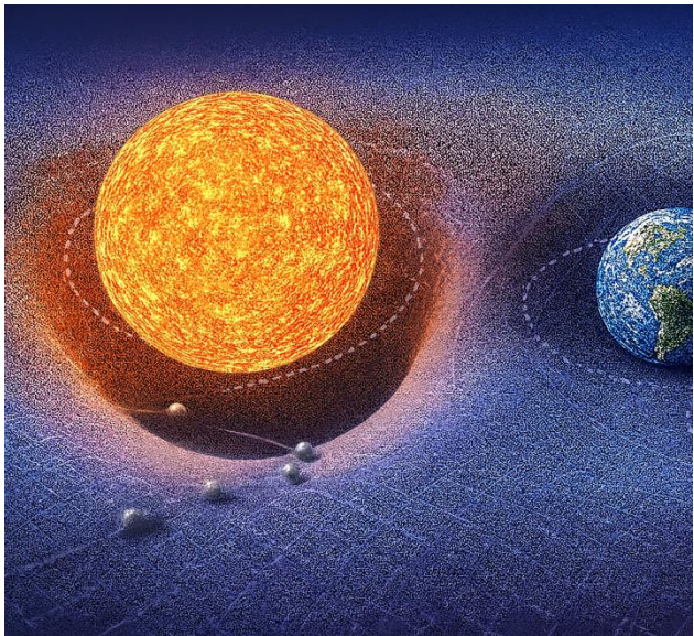
Traditional GR spacetime "rubber-sheet" model
