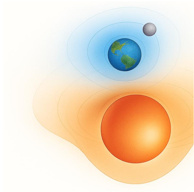
Gravity in G4D — curvature into a higher spatial dimension
