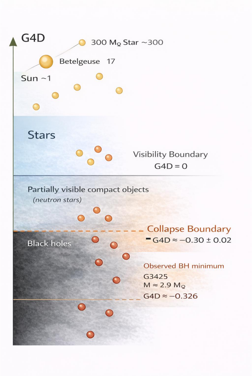
Conceptual illustration of the G4D visibility regimes. Objects with G4D > 0 remain fully visible, compact objects appear in the partially visible band between G4D = 0 and the collapse boundary, and black holes occupy the regime below G4D \approx -0.30 where gravitational confinement dominates. (Illustration generated with AI assistance.)
