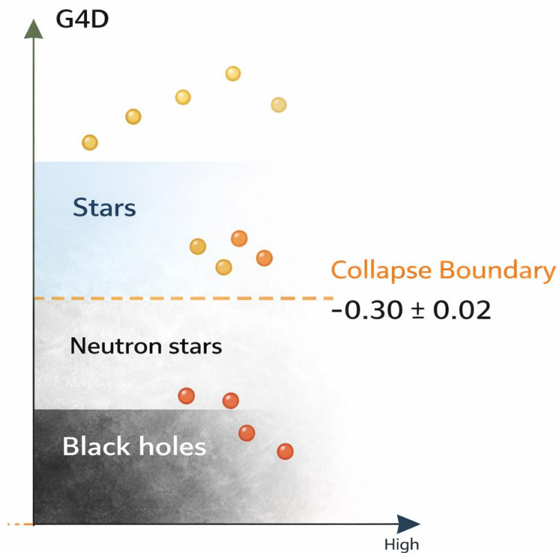
Conceptual illustration of the G4D visibility regimes. (Illustration generated with AI assistance.)
