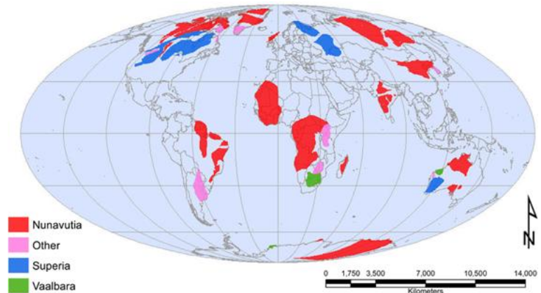
Present-day distribution of exposed Archean cratons and inferred supercratons (including Vaalbara), after open-source geological compilations. Source: Wikimedia Commons, CC BY-SA; based on published craton reconstructions.
