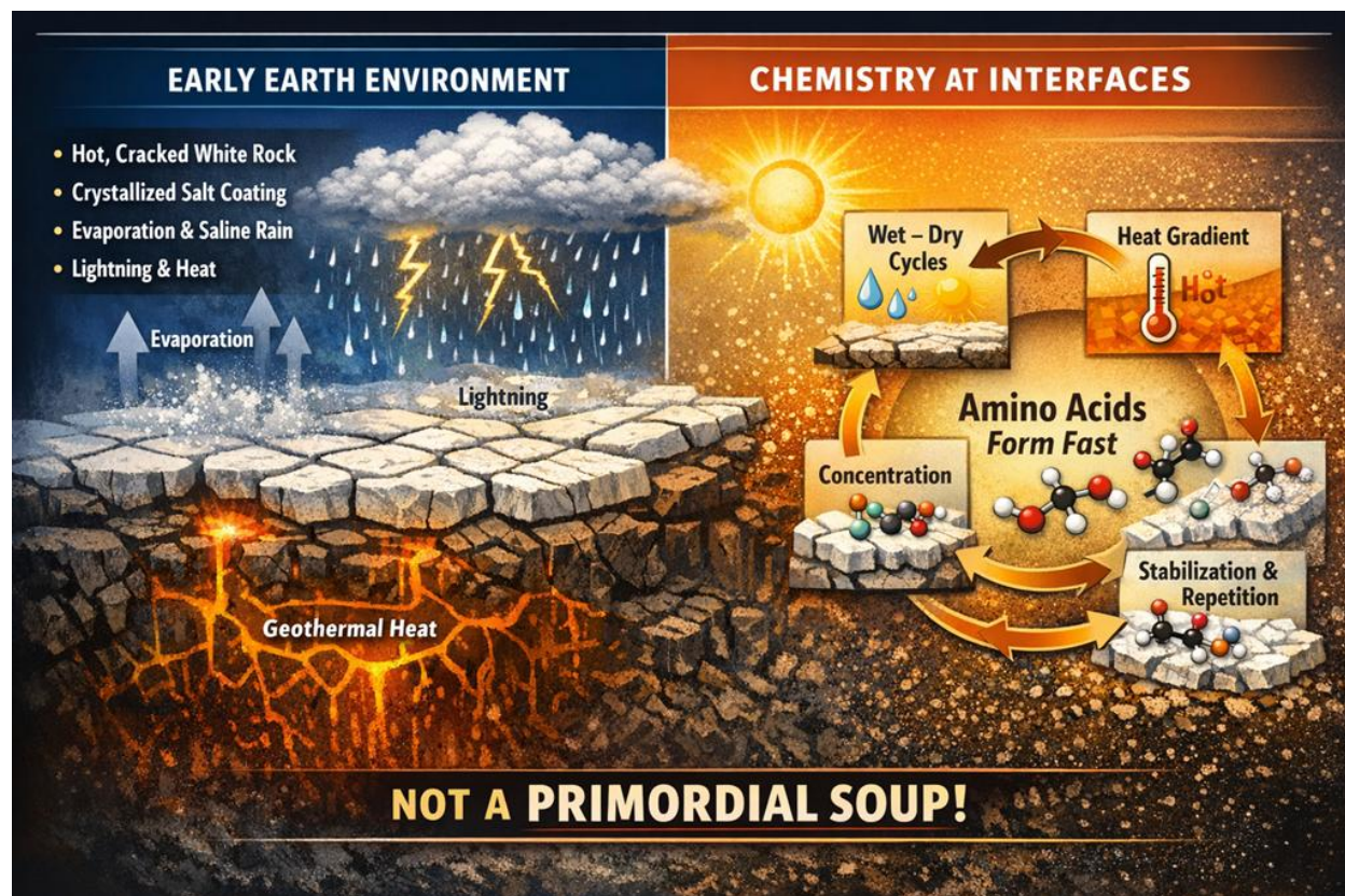
Figure 9.6 — Early Earth as a global chemical reactor - conceptual synthesis based on established early Earth geochemistry. (AI-generated conceptual illustration, AI-assisted generation)
