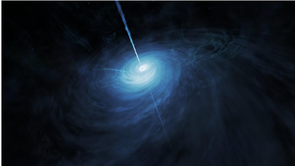
Artistic representation of quasar J043947.08+163415.7 (Image: ESA/Hubble, NASA, M. Kornmesser)
