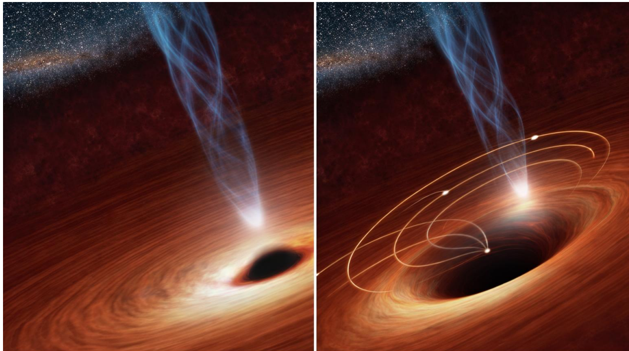
Classical depiction: Compact object with a "surface"
