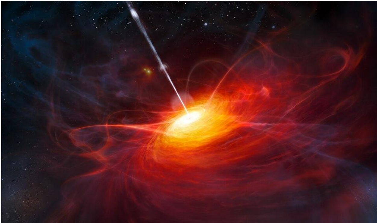
Artist's impression of the distant quasar ULAS J1120+0641 (Image credit: ESO / M. Kornmesser)
