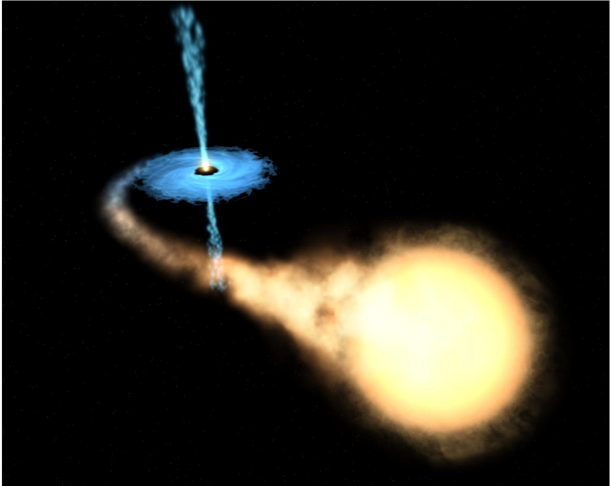
Artist's impression of the microquasar GRO J1655–40, showing a stellar-mass black hole accreting matter from a companion star, forming an accretion disk and relativistic jets. Credit: NASA / ESA (Hubble Space Telescope).
