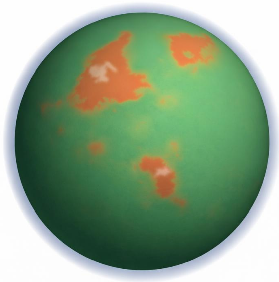
Early Archean
