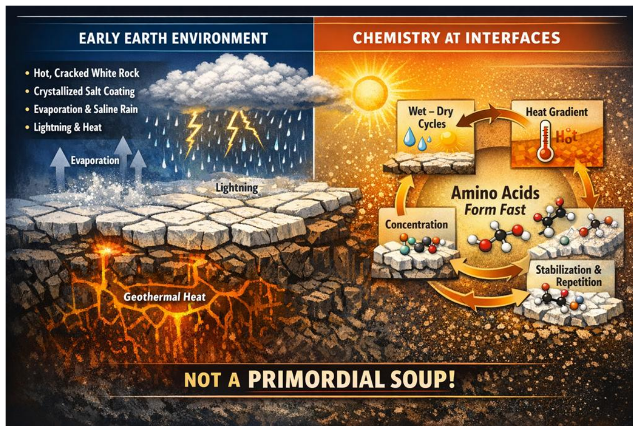
Figure 9.1 — Early Earth as a global chemical reactor - conceptual synthesis based on established early Earth geochemistry. (AI-generated conceptual illustration, created with ChatGPT 5.2)
