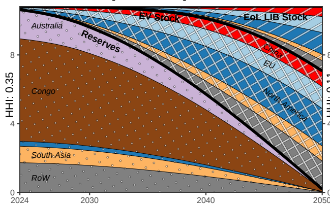
(c) Cobalt Stock [million tons]
