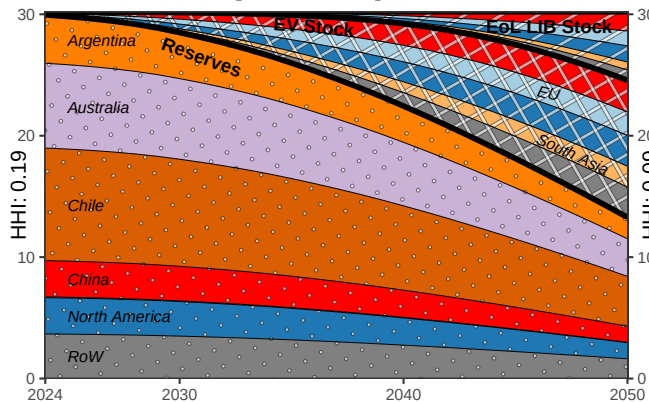
(a) Lithium Stock [million tons]
