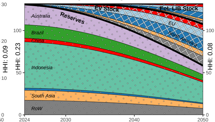
(b) Nickel Stock [million tons]
