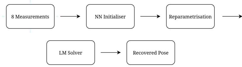
Figure 2.5: Data pipeline for hybrid model
