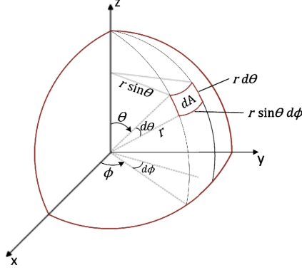
Figure 2.3: Area element on the unit sphere. Reproduced from [1]
