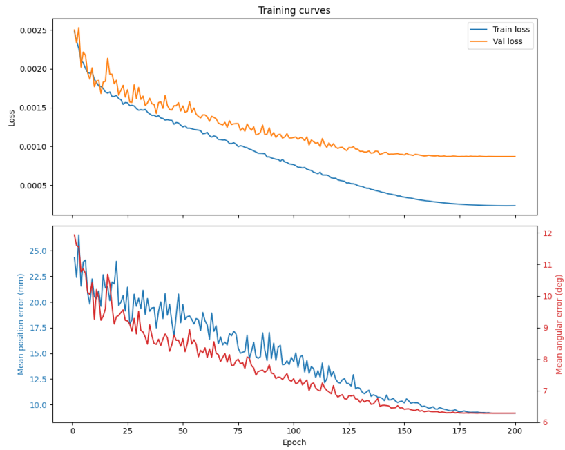
Figure 3.3: Loss curves and error curves on the validation set
