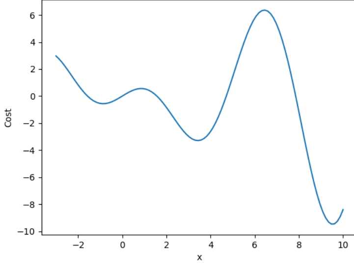
Figure 2.2: Example showing multiple local minima using y = x \cos x , x \in (-3, 10)
