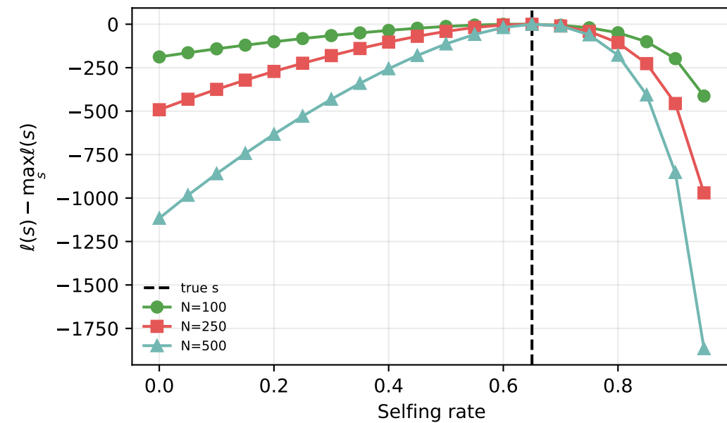
F. n=6, relative likelihood
