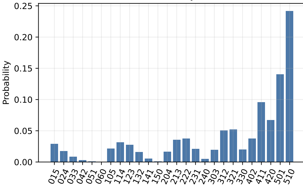
D. n=6, analytical
