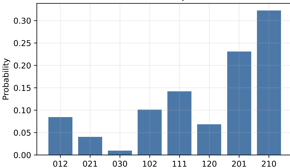
A. n=3, analytical
