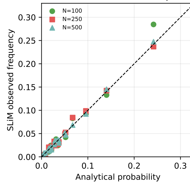
E. n=6, observed vs analytical
