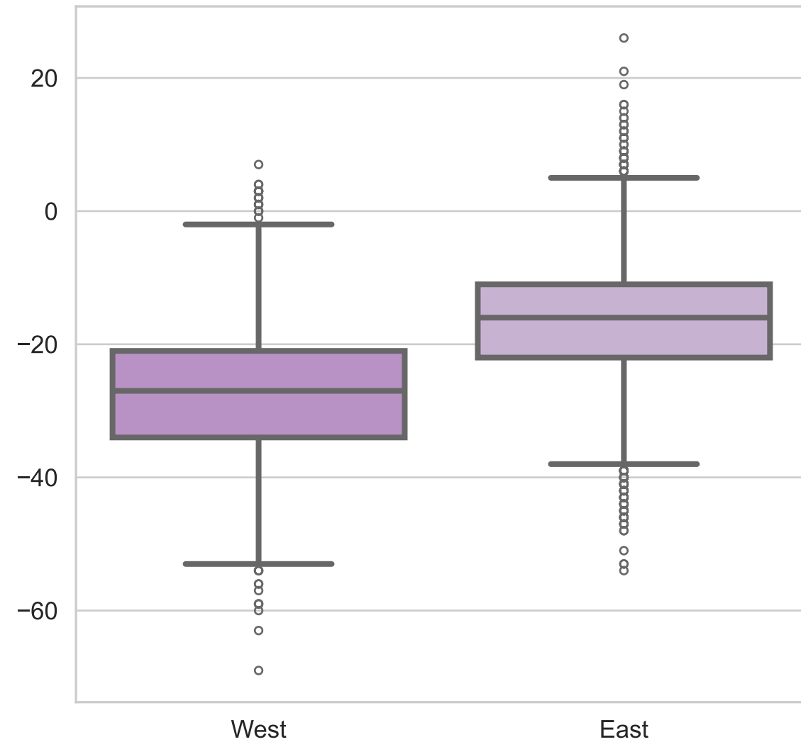
Blue-Yellow (b)
