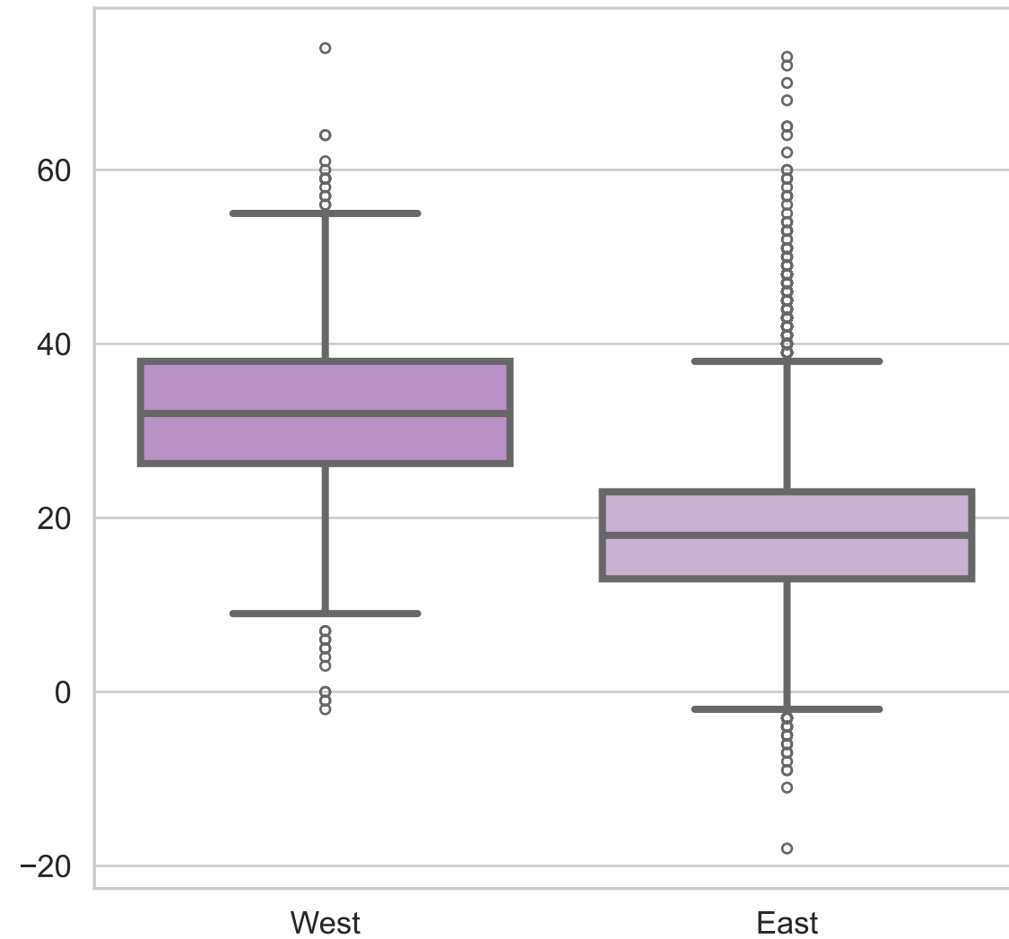
Green-Red (a)
