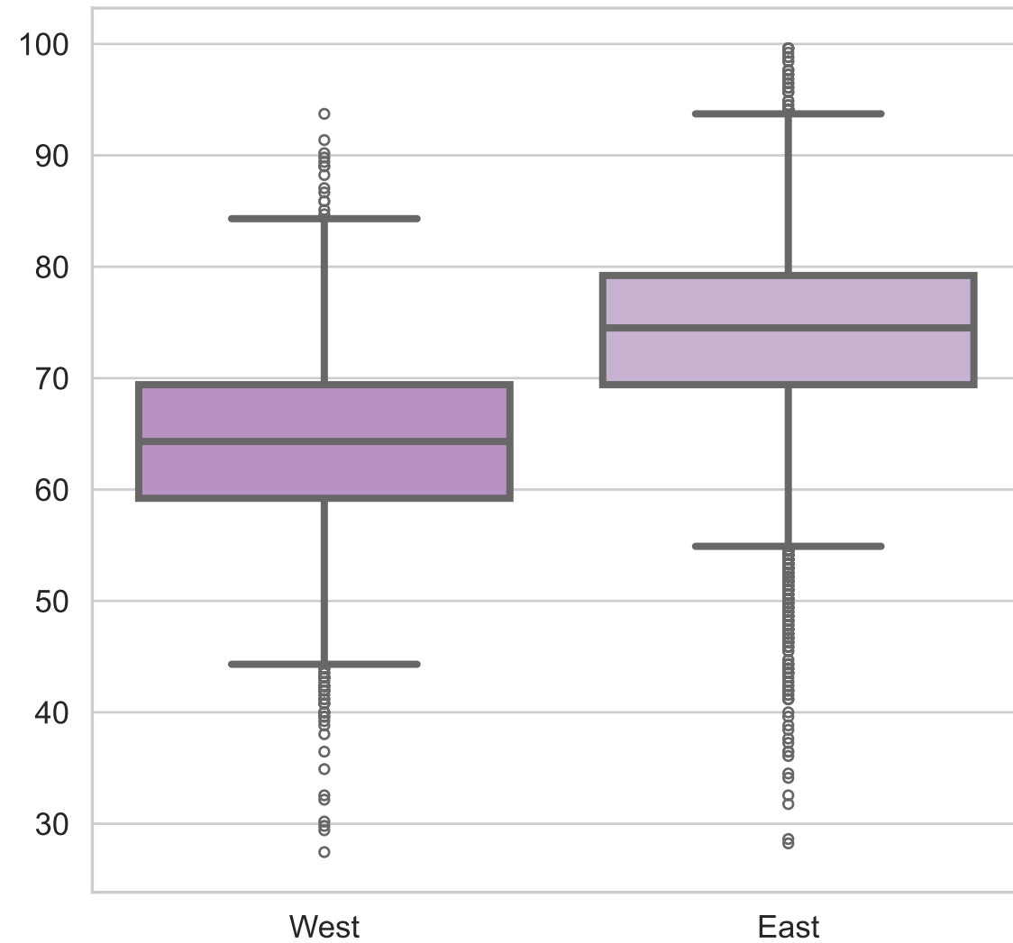
Lightness (L)
