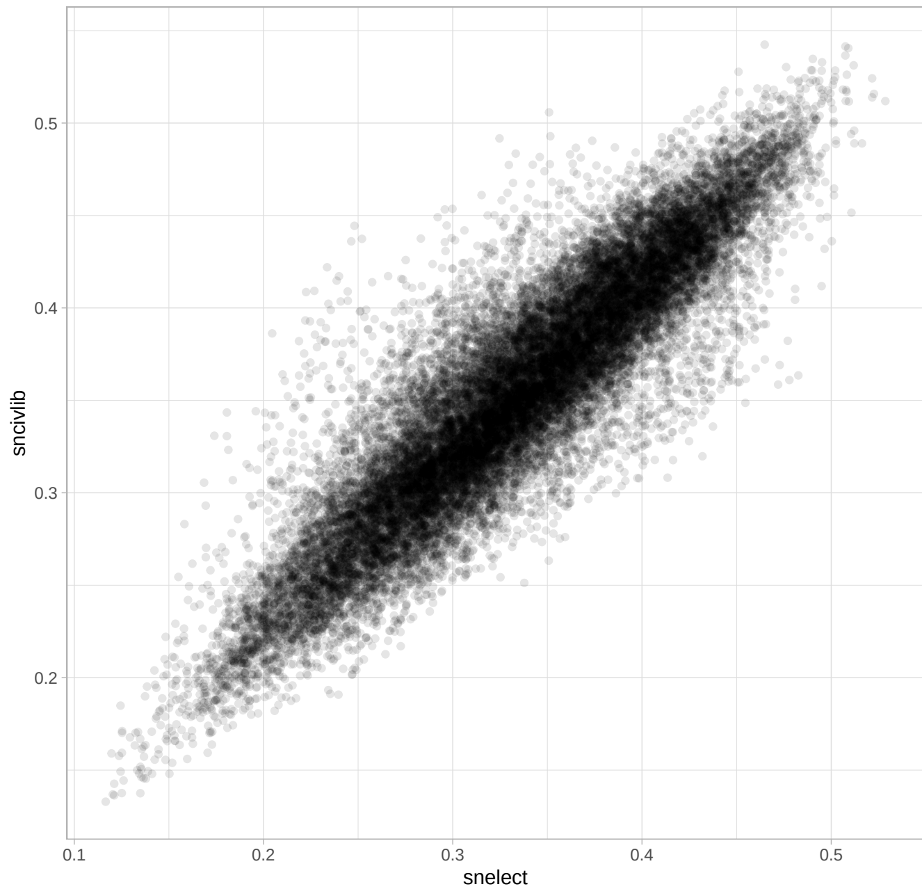
Electoral vs. Civil Liberties Index (pre-benchmarking)
