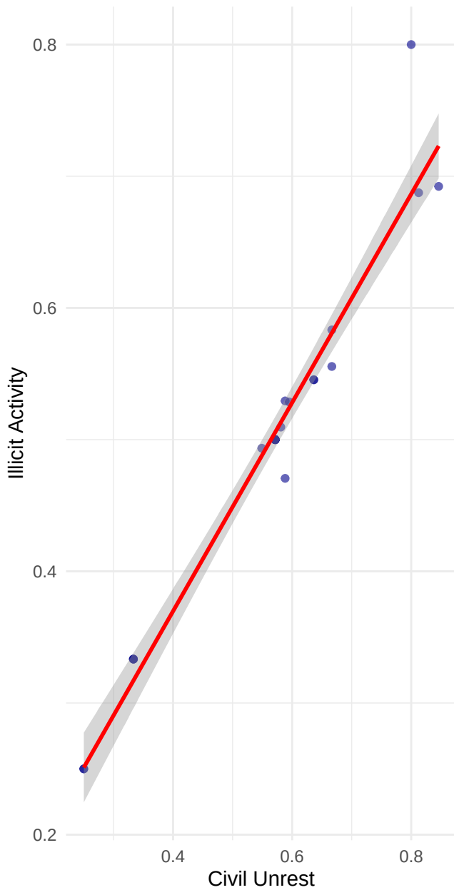
Elections (el) Components
