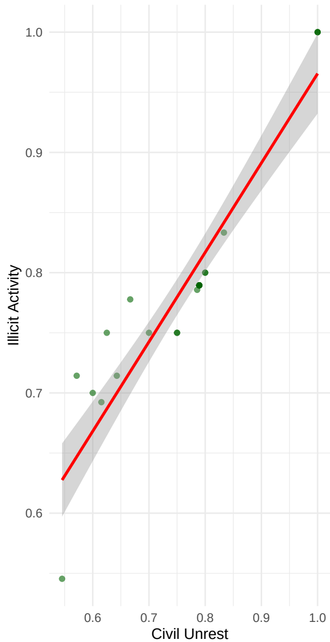
Civil Liberties (cl) Components
