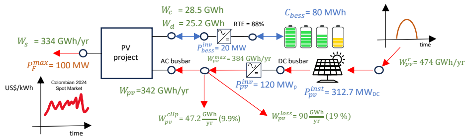
Figure 6: Annual energy balance of the project.
