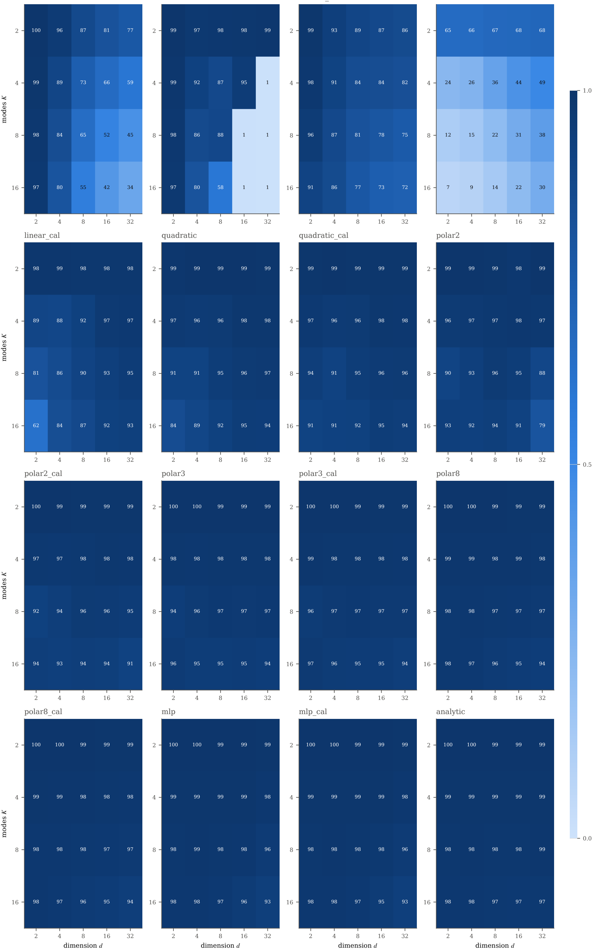
kernel overall accuracy (%) — best anchor budget per cell, true-score T=100
