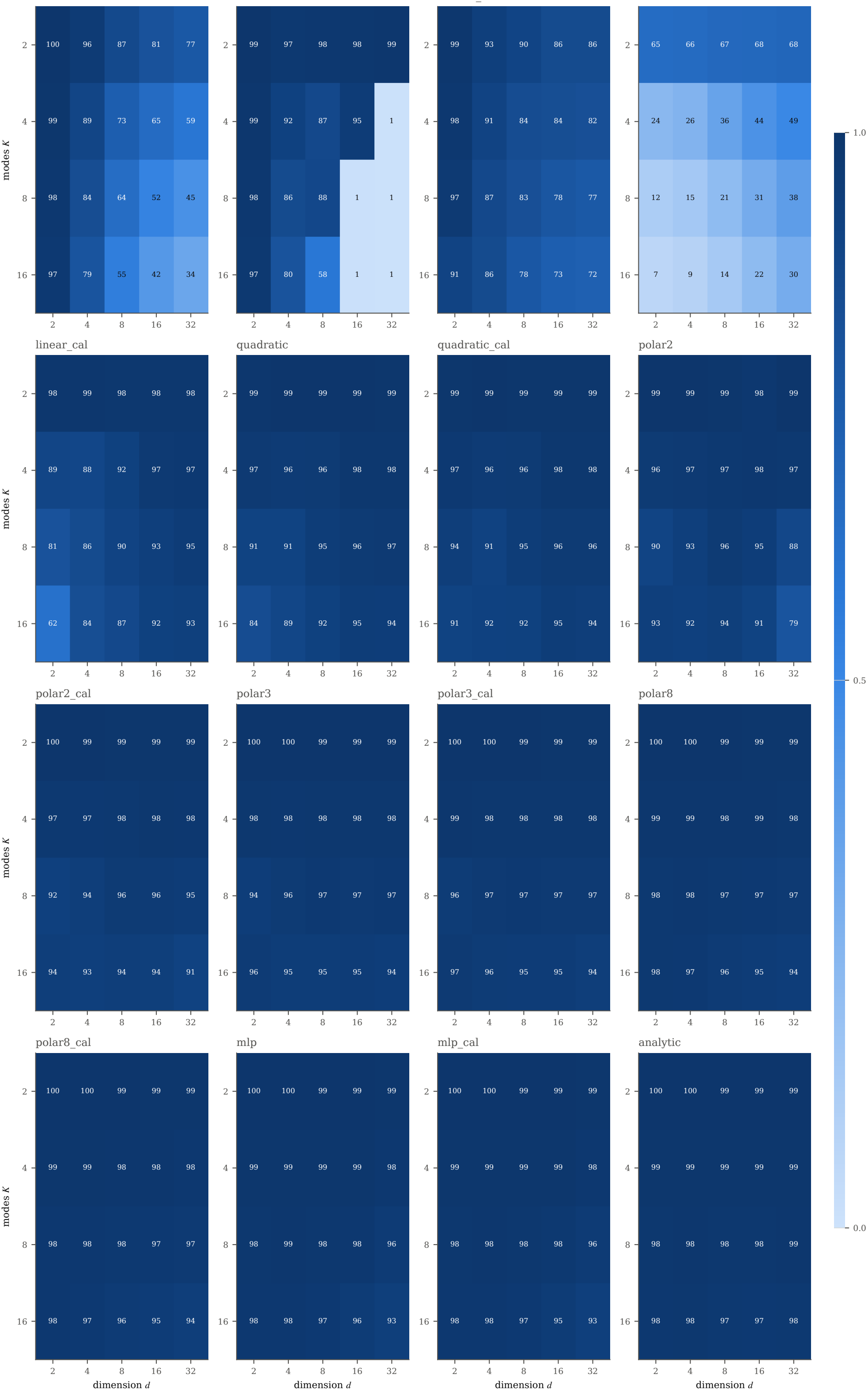
kernel overall accuracy (%) — best anchor budget per cell, true-score T=500
