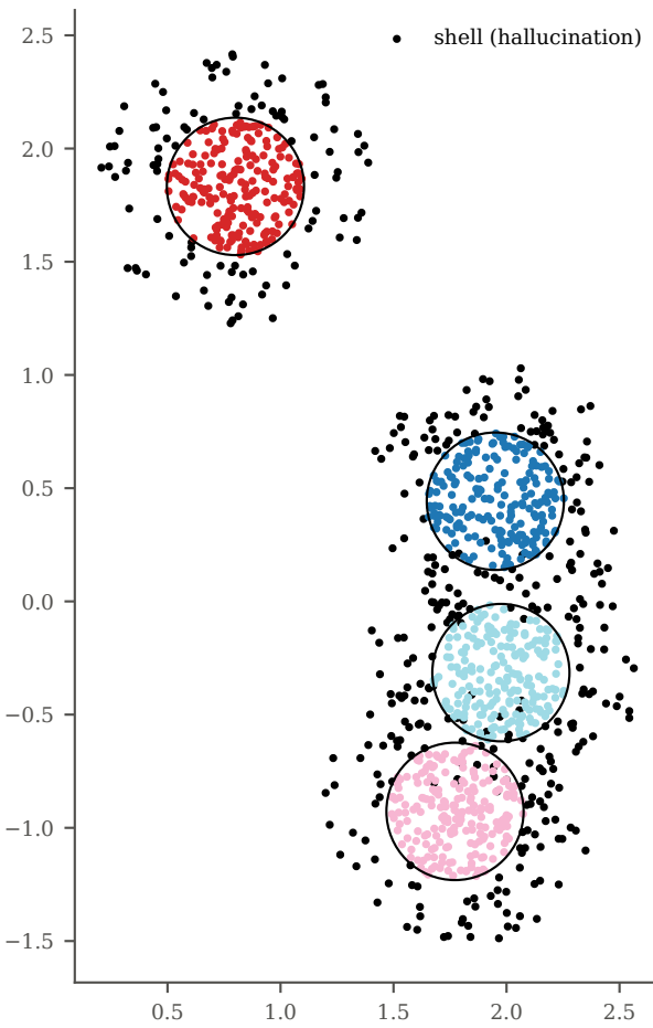
anchors in DATA space (K=4): 800 disk + 400 shell
