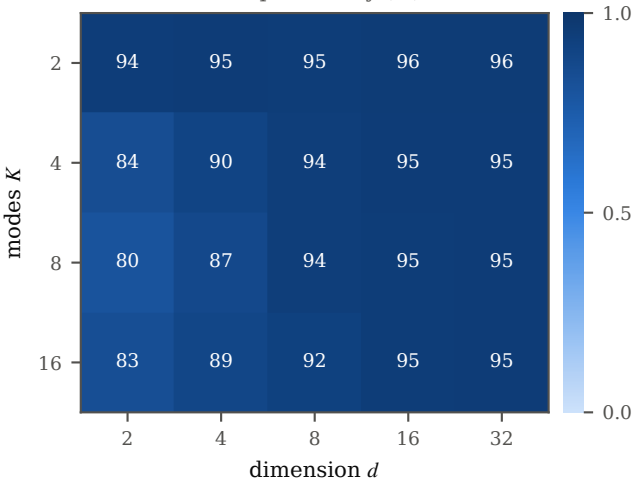
anchor round-trip accuracy (%), T=100
