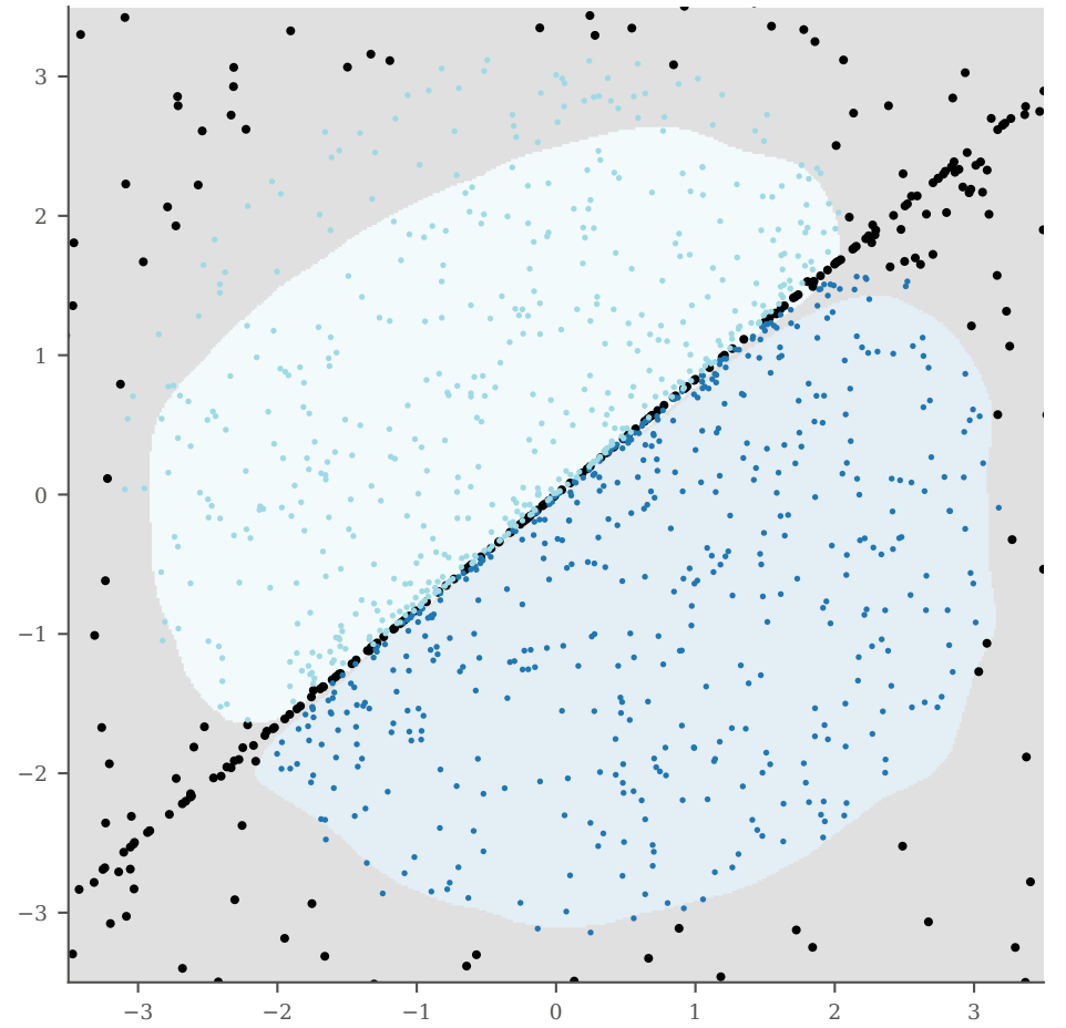
backtracked to SEED space (true score, T=1000) over the learned fate map
