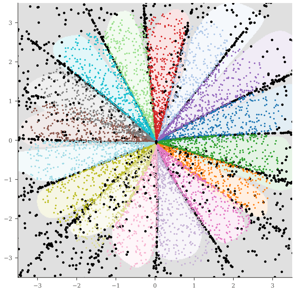
backtracked to SEED space (true score, T=150) over the learned fate map
