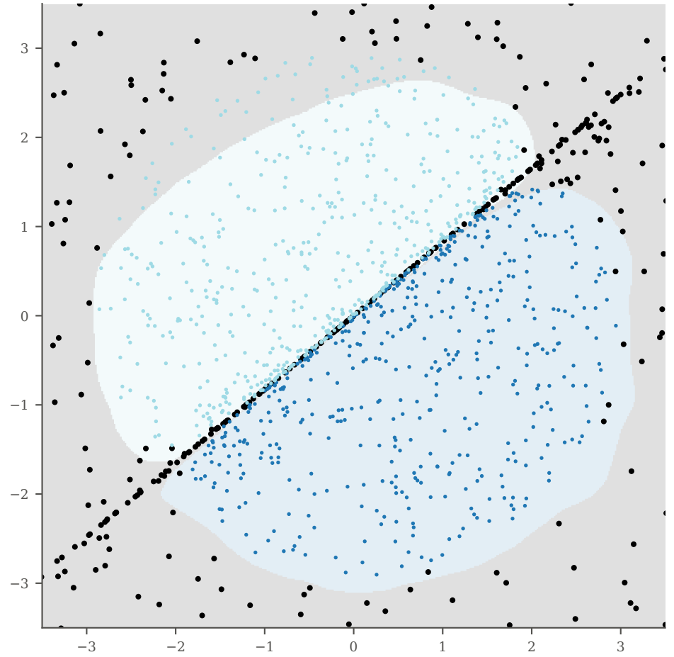
backtracked to SEED space (true score, T=150) over the learned fate map
