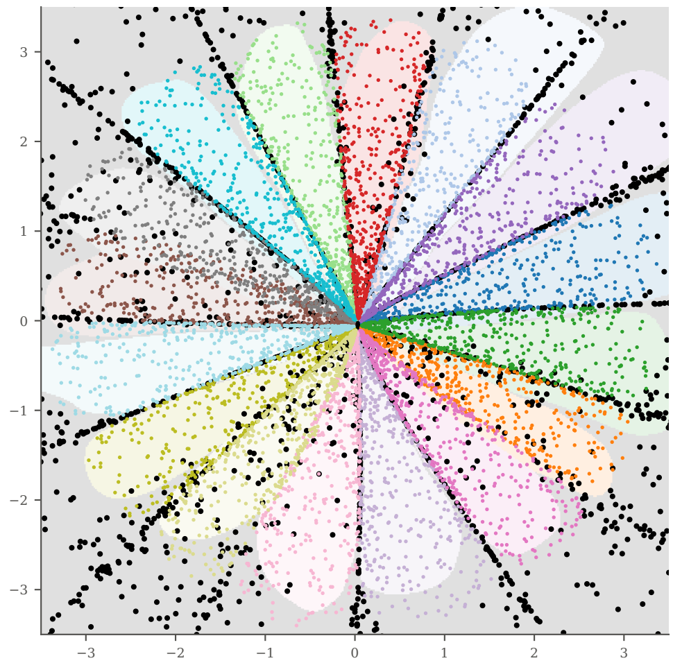
backtracked to SEED space (true score, T=300) over the learned fate map
