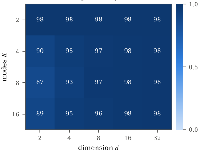
anchor round-trip accuracy (%), T=400
