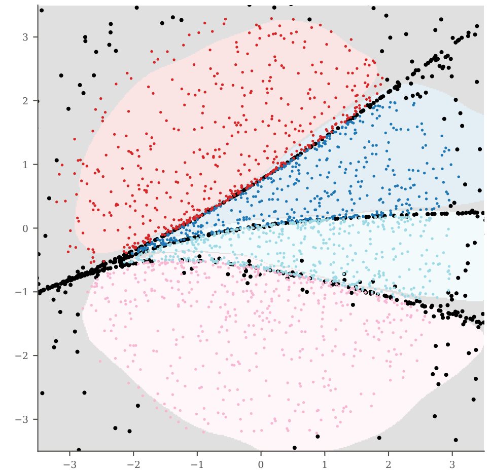
backtracked to SEED space (true score, T=700) over the learned fate map
