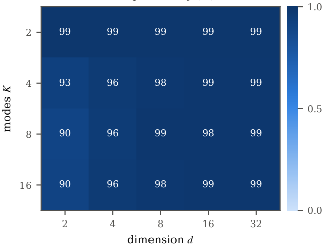
anchor round-trip accuracy (%), T=750
