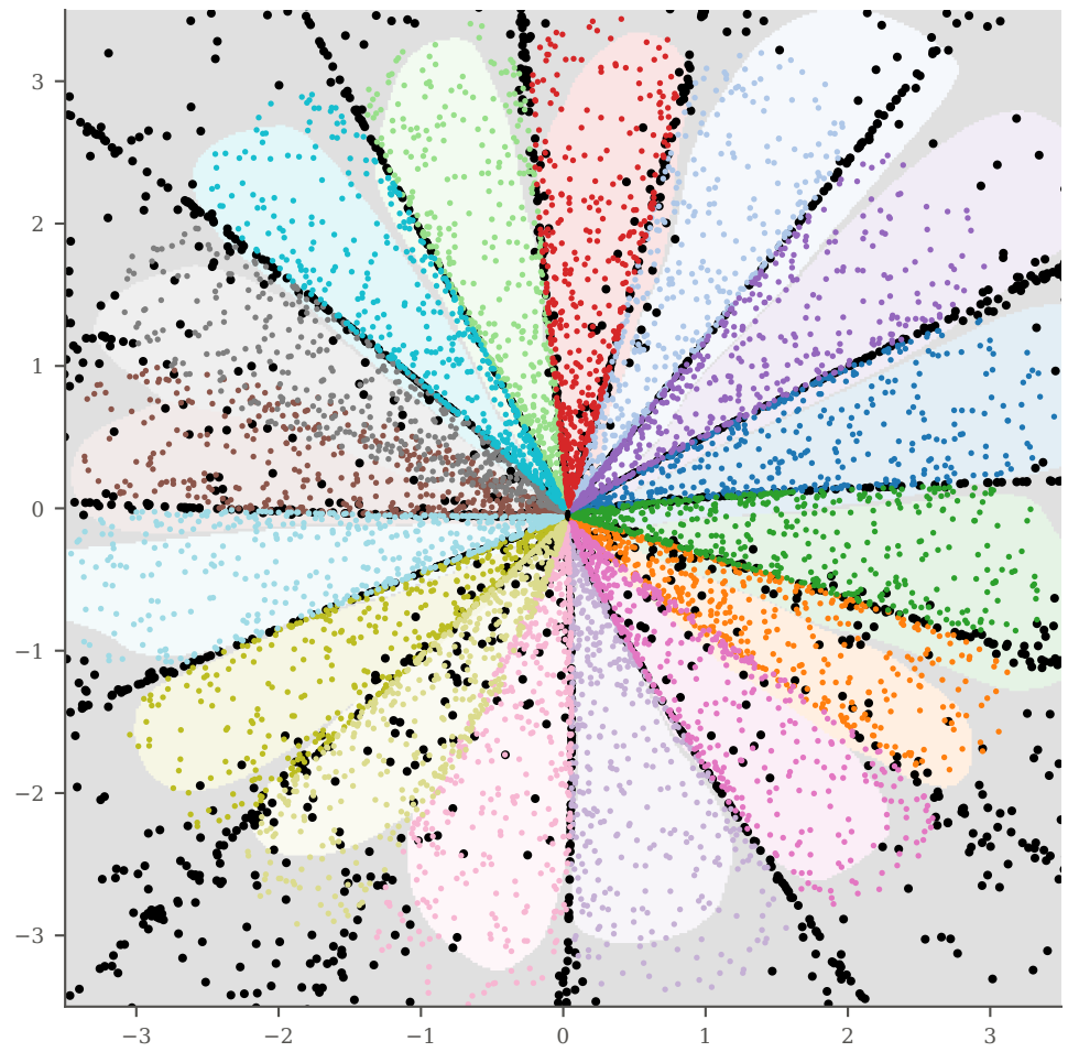
backtracked to SEED space (true score, T=800 ) over the learned fate map
