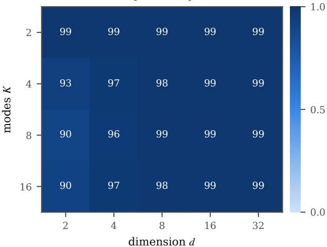
anchor round-trip accuracy (%), T=800
