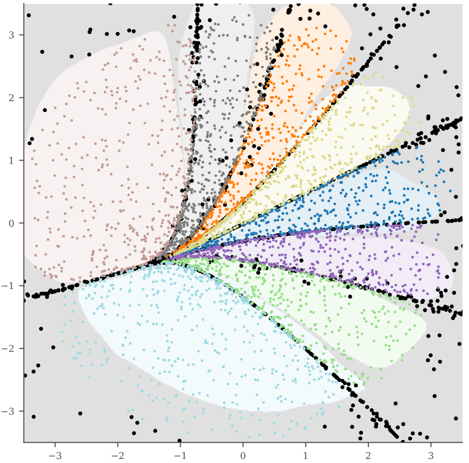
backtracked to SEED space (true score, T=950) over the learned fate map
