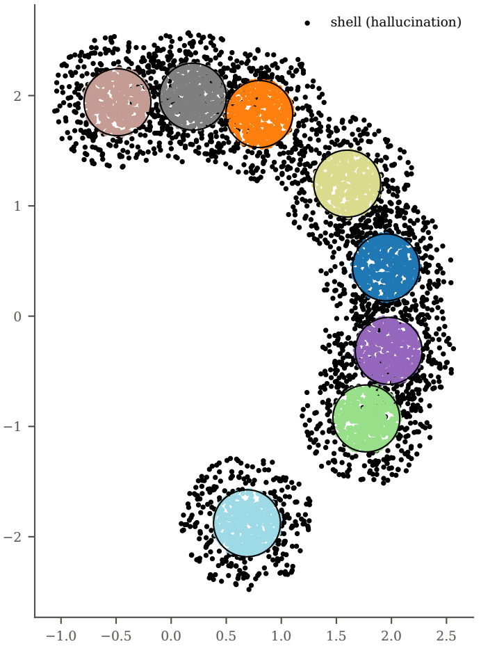
anchors in DATA space (K=8): 4000 disk + 2000 shell
