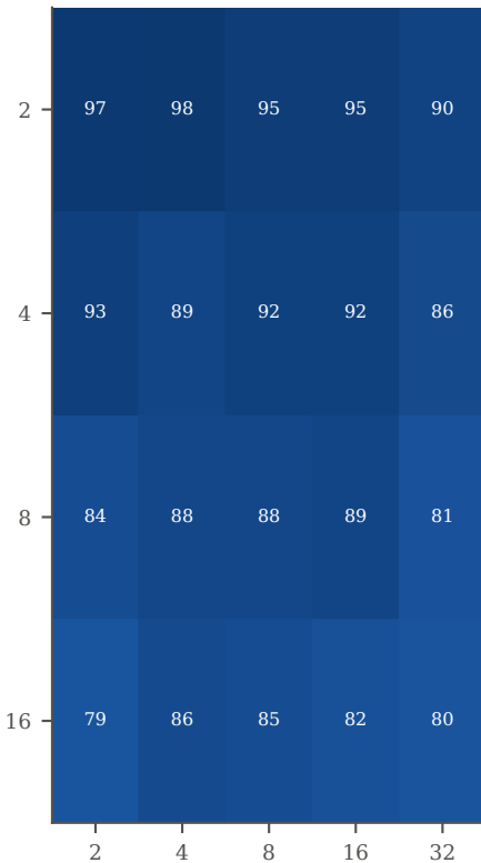
analytic
