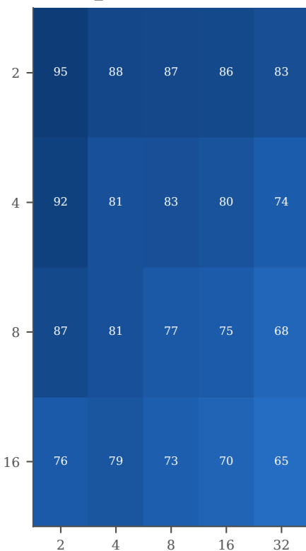
polar2
