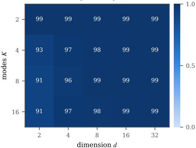
anchor round-trip accuracy (%), T=950
